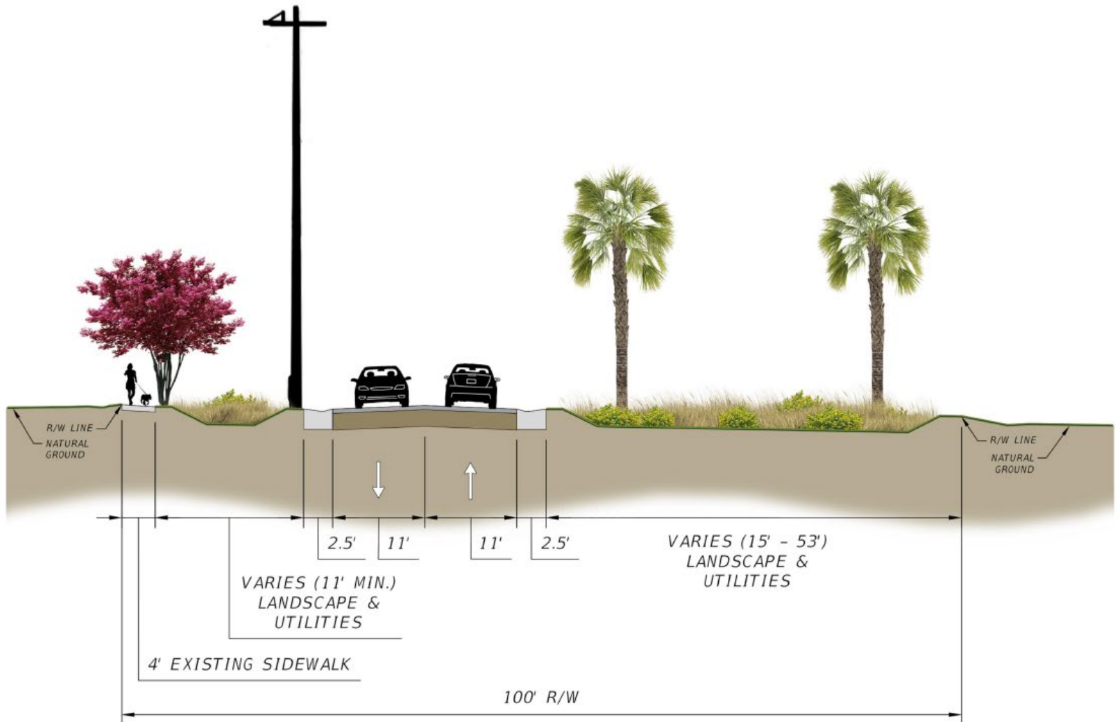
Typical Section (A-A') West End to Park Drive
