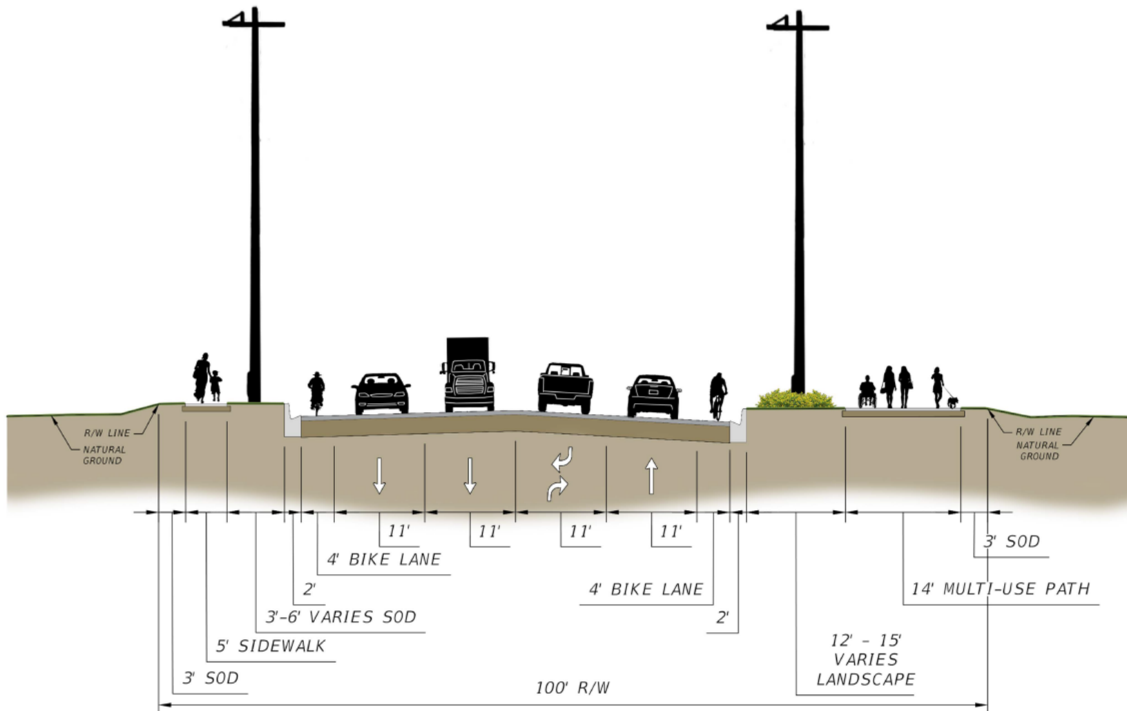
Typical Section (D-D') 1st Beach Park to Driveway
