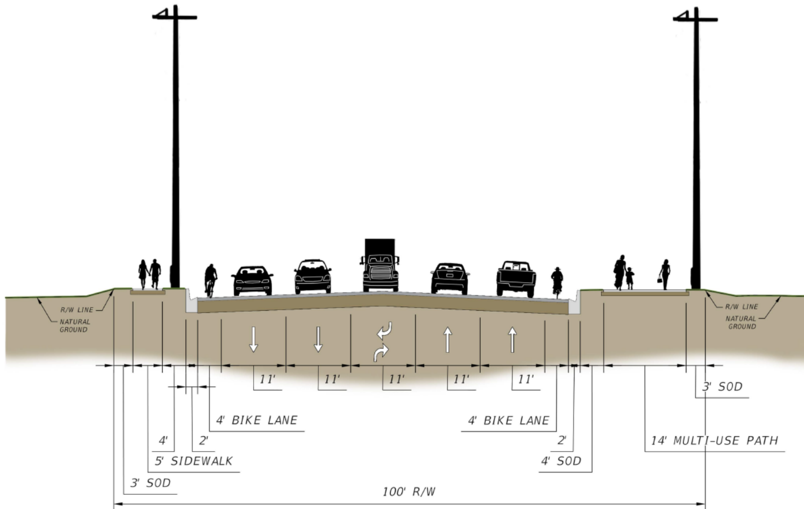
Typical Section (E-E') Driveway to Brooks Bridge
