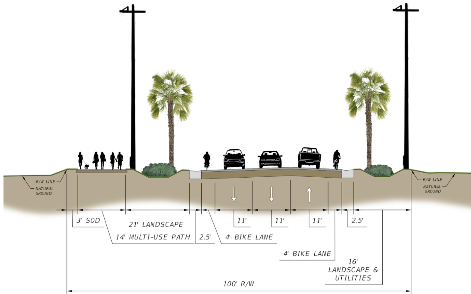
Typical Section (C-C') 4th Beach Park to 1st Beach Park
