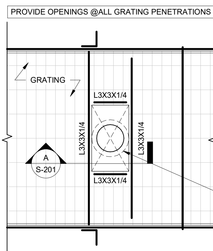
4 GRATING OPENING DETAIL 1" = 1'-0"
