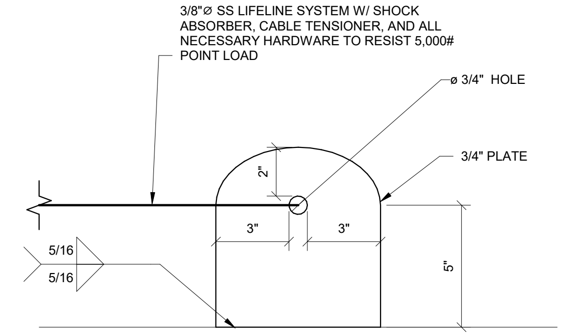
2 BID OPTION - FALL PROTECTION PAD EYE 3" = 1'-0"
