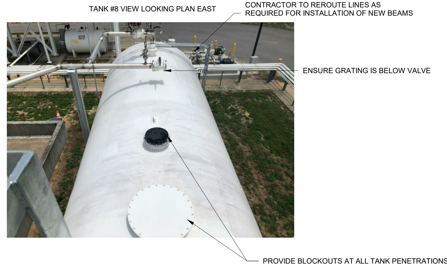
1 TANK #8 PLAN EAST VIEW 3/4" = 1'-0"
